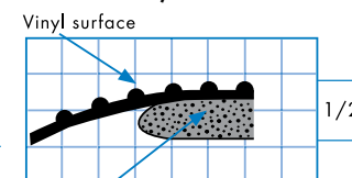
Flex-Link™ sponge base
